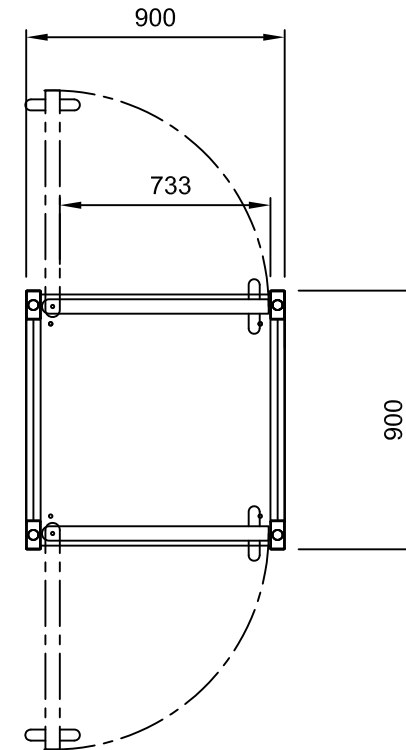
PLAN VIEW © TURNSTAR SYSTEMS
