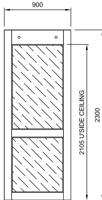
SIDE ELEVATION © TURNSTAR SYSTEMS
