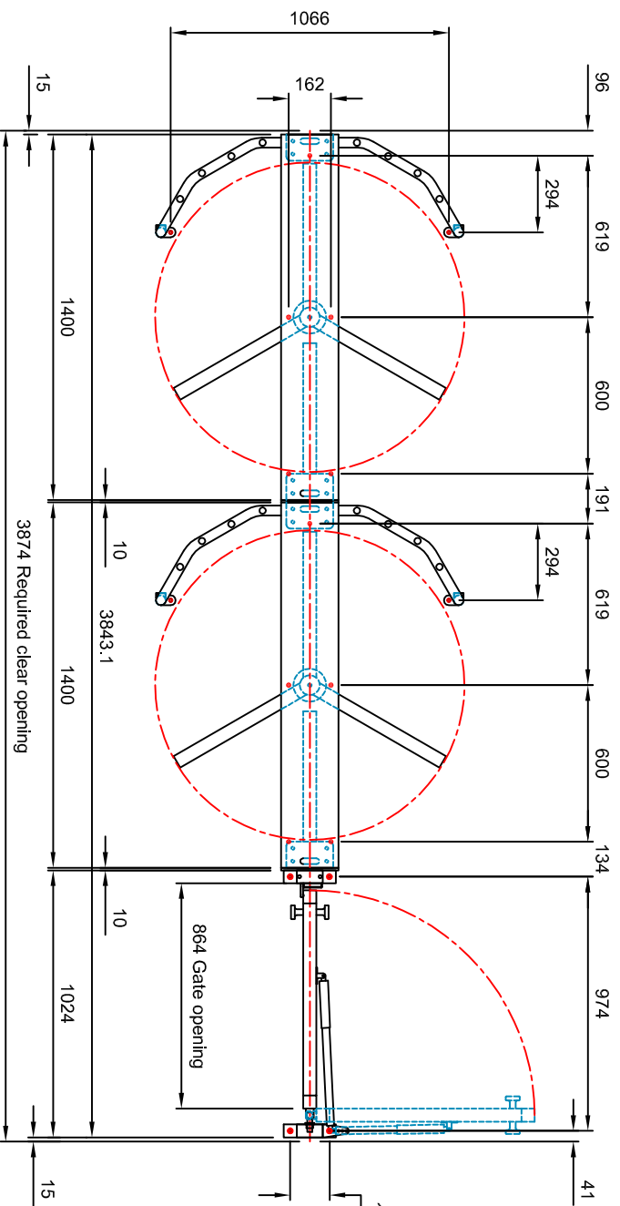
PLAN VIEW
