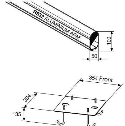
ANCHORAGE PLATE 354x304 with M14x200 log bolts
