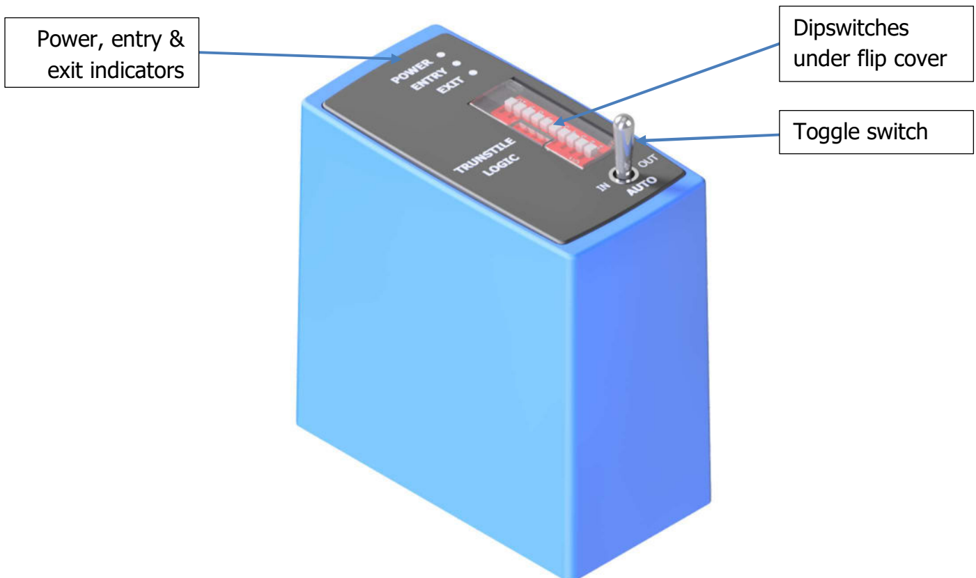
Figure 24: Blue Plug-in Logic (TL300TUR)
