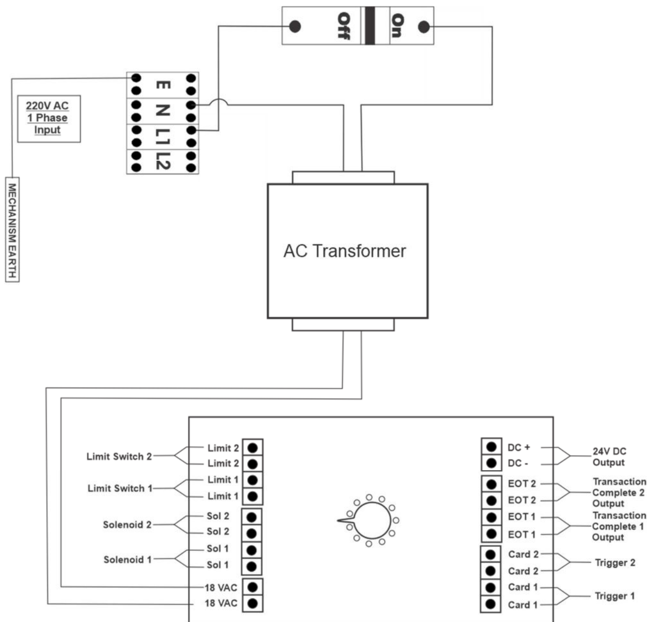
Figure 25: Wiring Diagram for Full Height Turnstile
