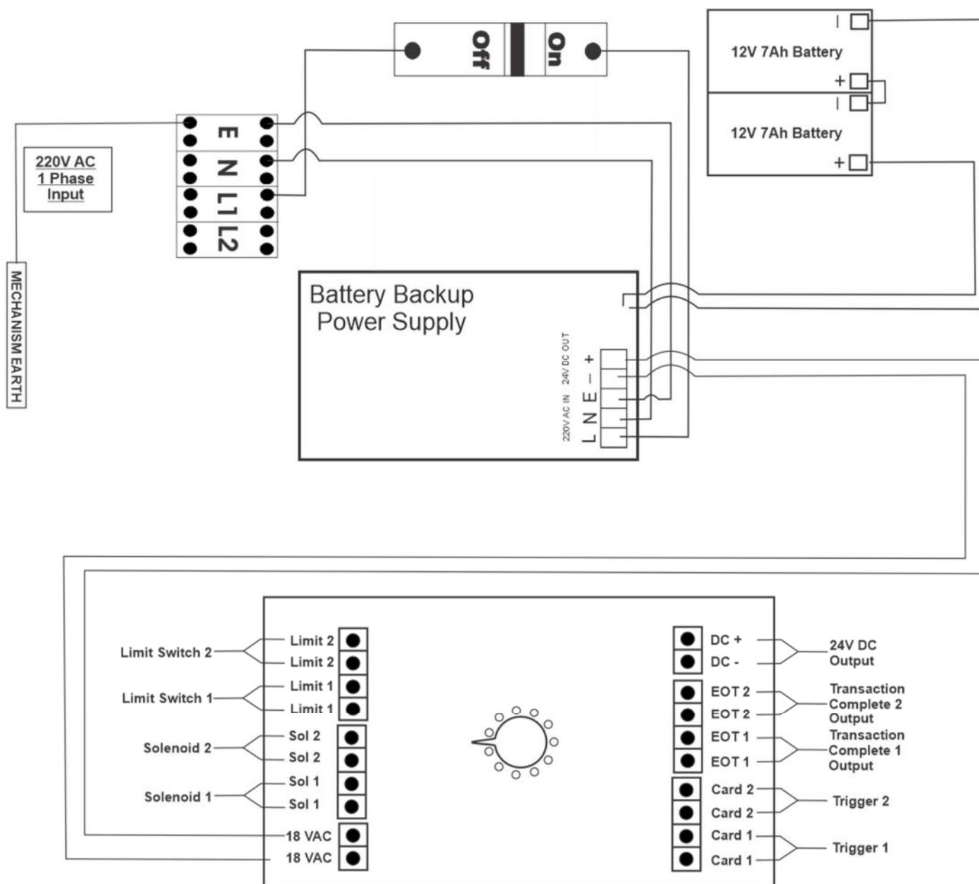
Figure 26: Wiring Diagram for FH Turnstile with Battery Backup
