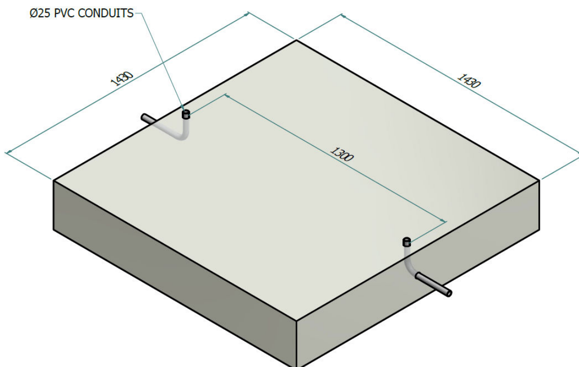
Figure 23: Isometric view on plinth and conduits provision
