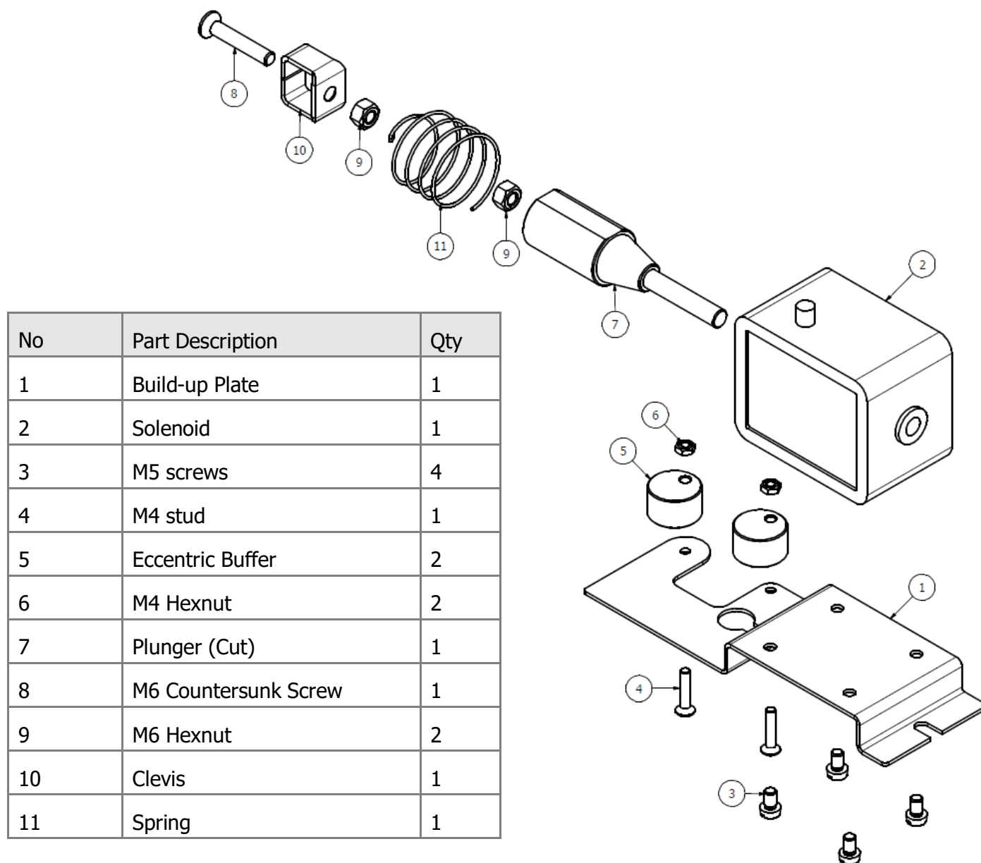
Figure 29: Solenoid assembly – Fail-secure
