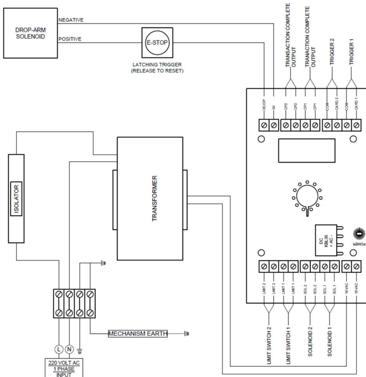
Figure 5: Wiring Diagram for Streamline Drop-Arm
