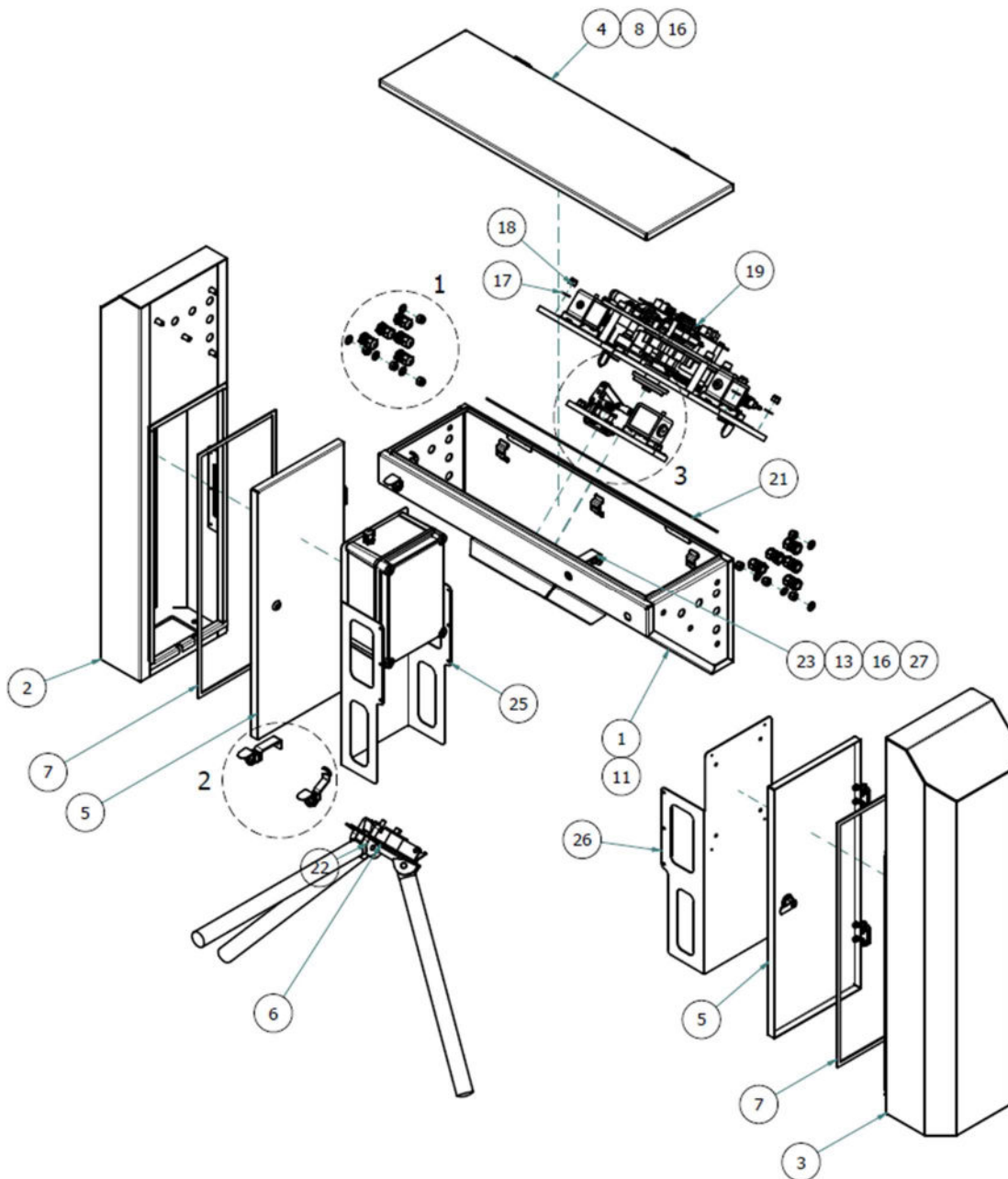
Figure 3: Exploded View of Streamline
