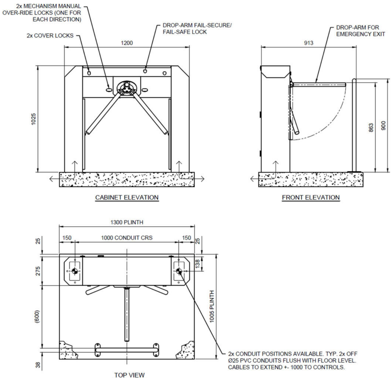
Figure 1: Layout of Streamline Drop-Arm
