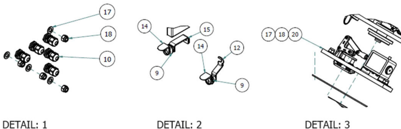
Figure 4: Details of Exploded View
