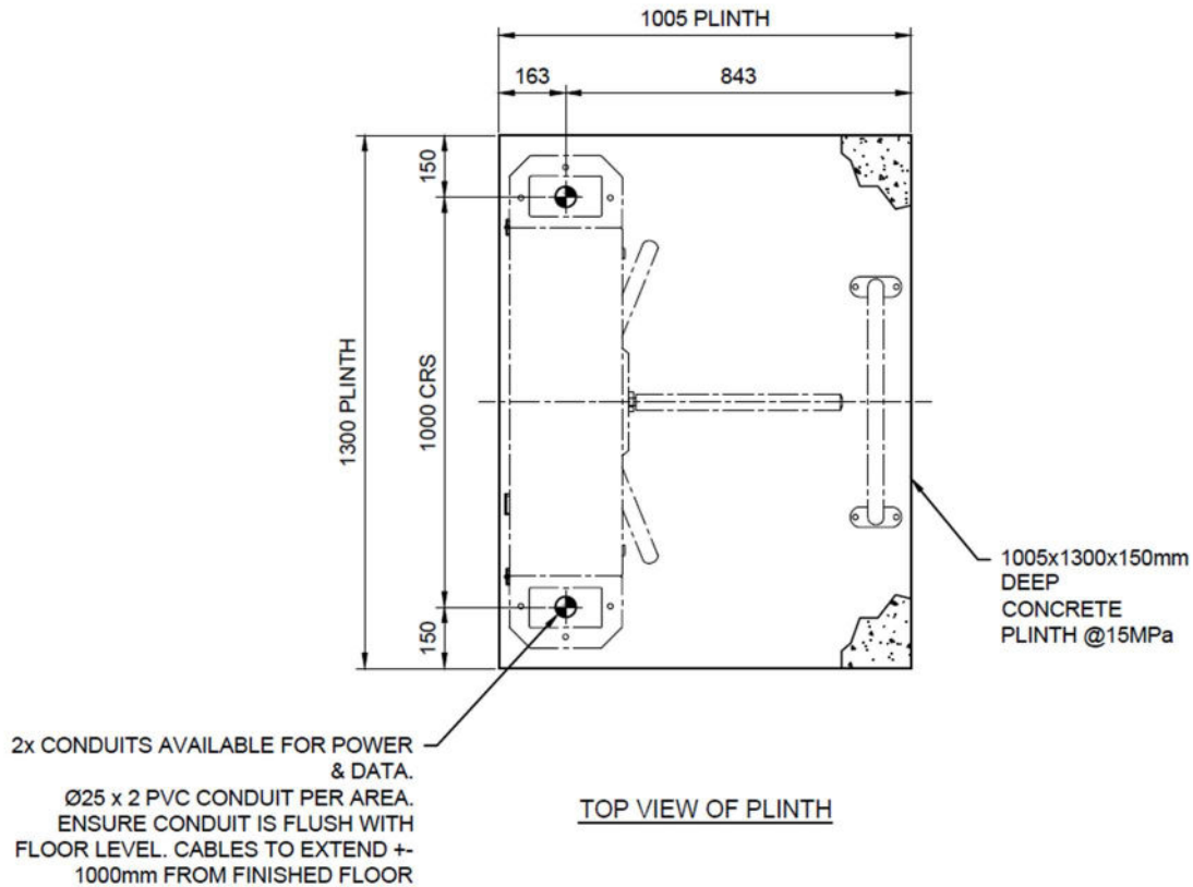
Figure 2: Top View of Plinth
